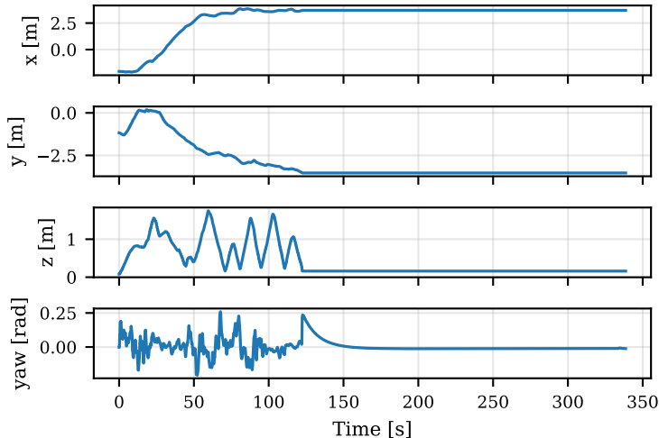
exp 5 - UAV 0 - Position
